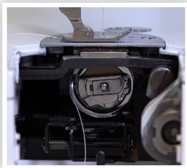
Vertical Full Rotary, Industrial Hook Bobbin
